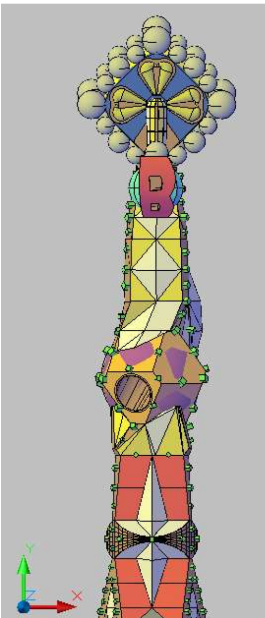
Figure 11 – The 3D model of the spire (plotting by D.Azzarone)
