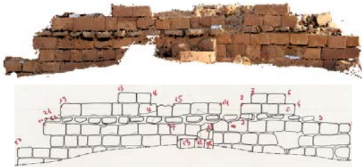
Fig. 18. Top: Meshed and textured point cloud. Bottom: Architectural man-made sketch of the external face of the wall of the building.
