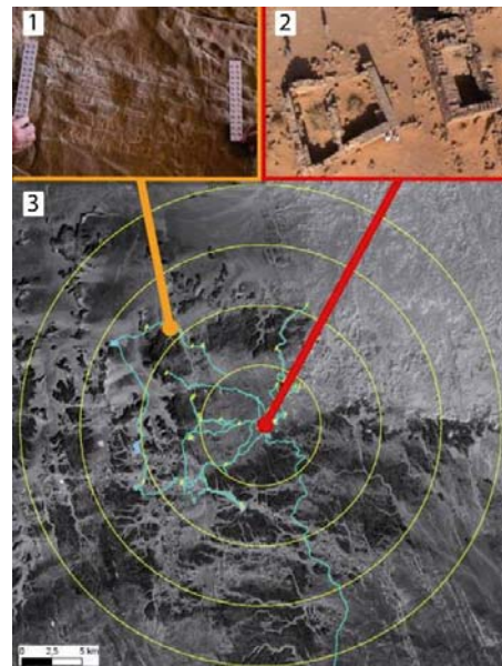
Fig. 7. Prospecting and excavating zones Sources: 1. Terrestrial Reflex camera image 2. Kite images from Geofil ® 3. Quickbird ® image.
